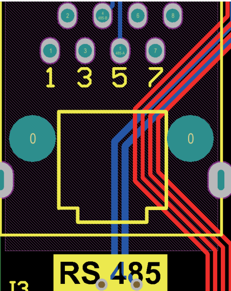
Porta RS 485
